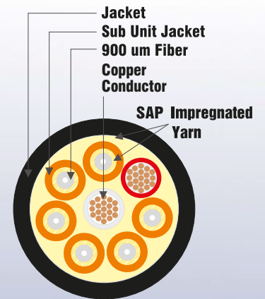
6 Fiber (Size Enlarged to show detail)
