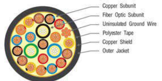
Example of a FTFA cable.
